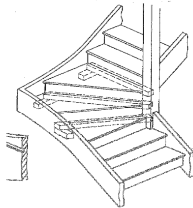
(60) Detail of winder support stringer
